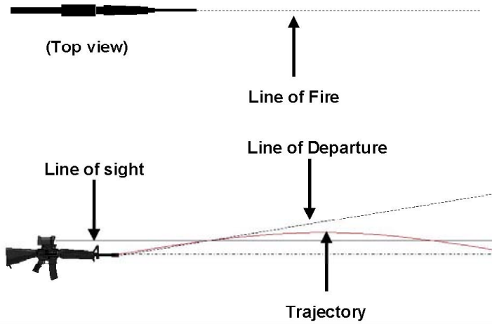
Figure 3-34a: Theory of Small Arms Fire
