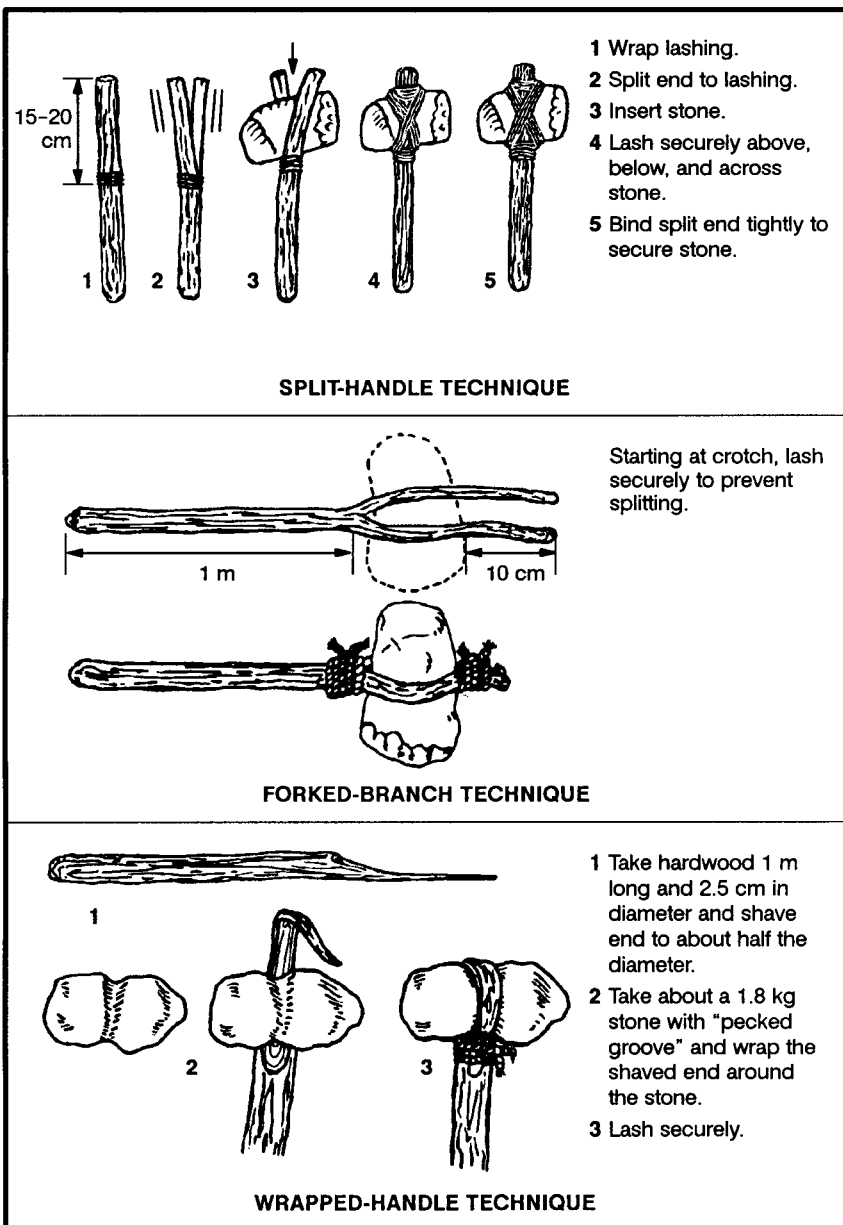
Figure 12-1. Lashing clubs.
